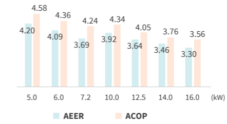
Cassette unit
